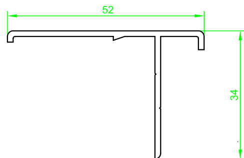
(ST 6935)"STARTEC" Geniş Kapama T Profili Ö:1/1 (ST 6935) "STARTEC" Wide T Covering Profile S:1/1
