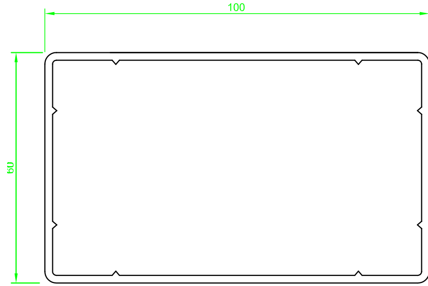
(ST 6990)"STARTEC" (100 x 60) Kutu Profili Ö:1/1 (ST 6990) "STARTEC" Rectangle Profile(100 x 60) S:1/1
