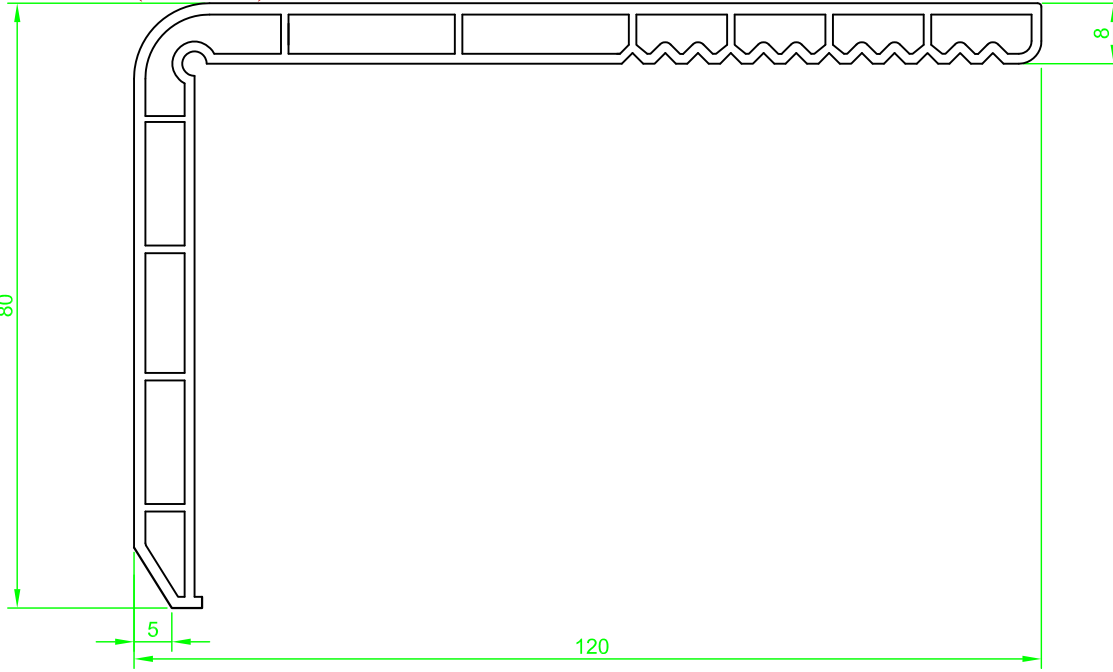
(ST 6950)"STARTEC" Pervaz Profili Ö:1/1 (ST 6950) "STARTEC" Sill Joint Extension Profile S:1/1
