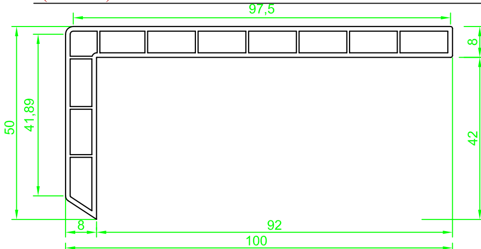
(ST 6940)"STARTEC" 5 X 10 Pervaz Profili Ö:1/1 (ST 6940) "STARTEC" 5 X 10 Sill Joint Extension Profile S:1/1
