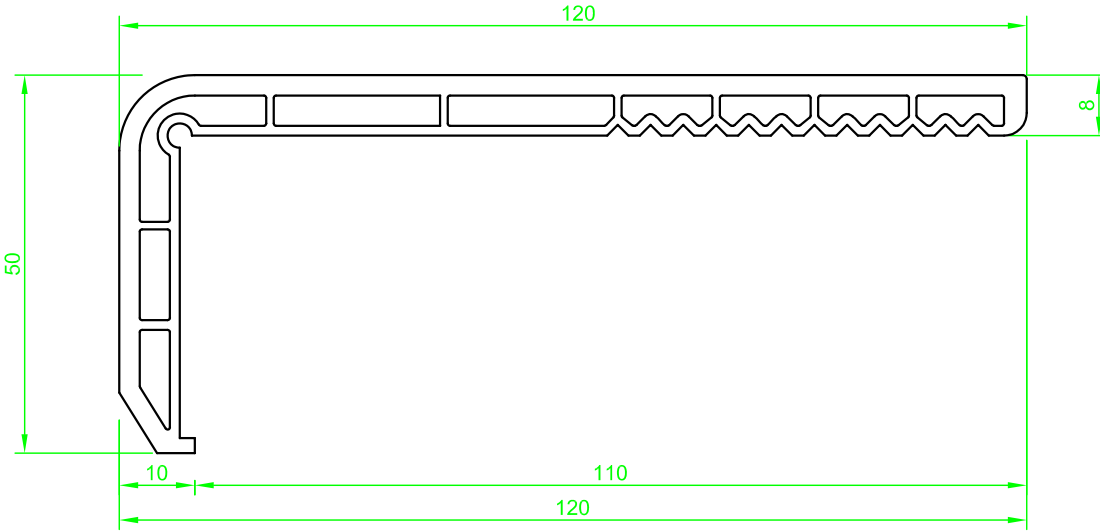
(ST 6950)"STARTEC" Pervaz Profili Ö:1/1 (ST 6950) "STARTEC" Sill Joint Extension Profile S:1/1
