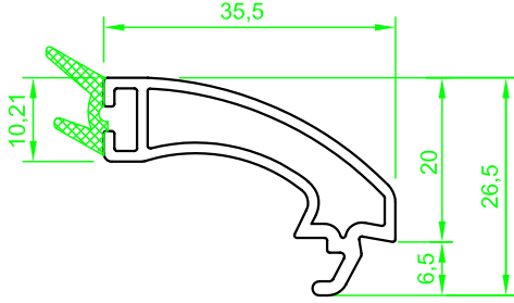
(ST 6530) "STARTEC Yap. Con.Dek. Tek Cam Çıtası" (ST 6530) "STARTEC Co-Extruded Dec. Single Glazing Bead"
